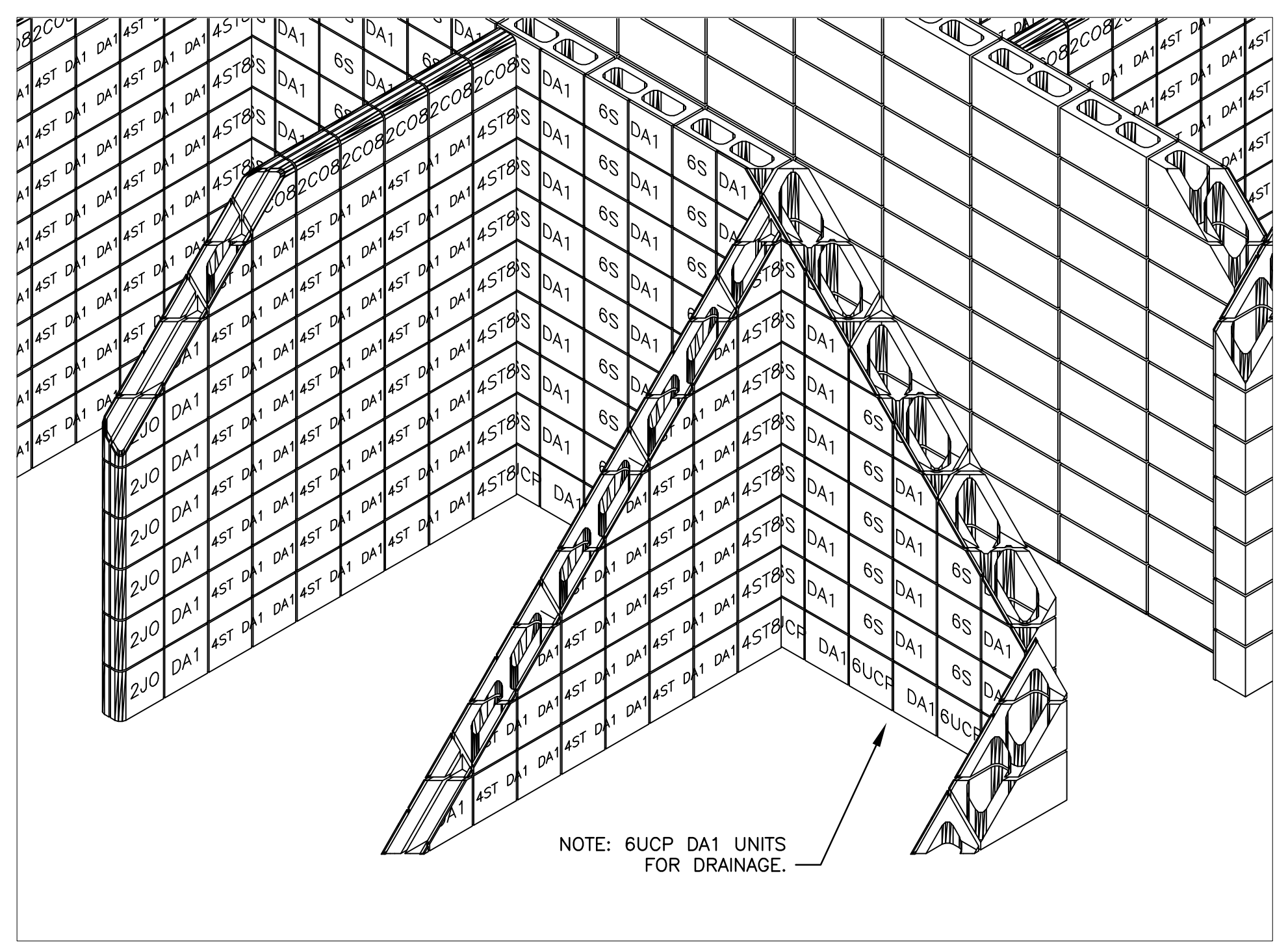
4 WALL DETAIL (CUT VIEW) SCALE: NONE REF:
