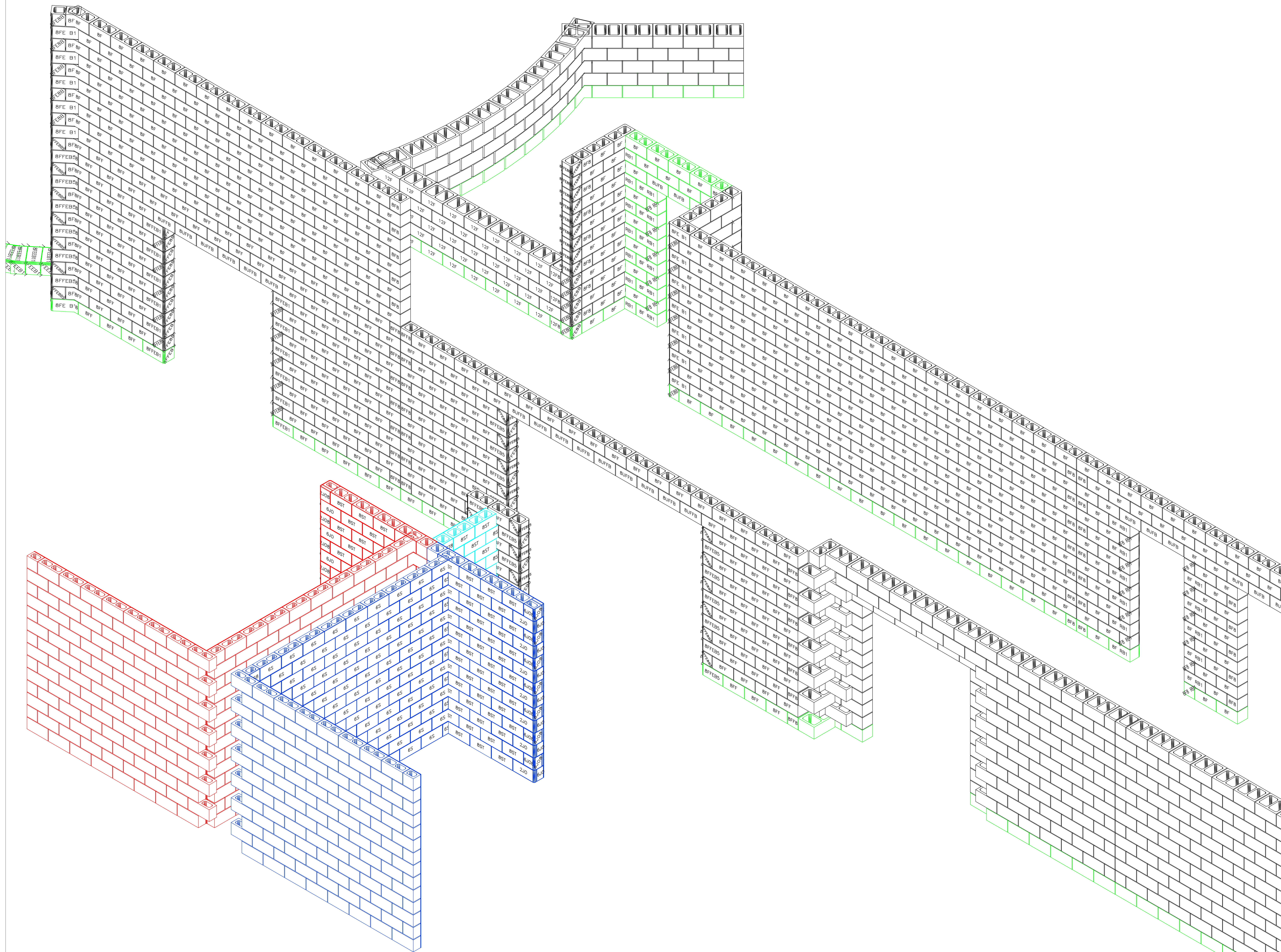
1 WALL DETAIL SCALE: NONE REF:
